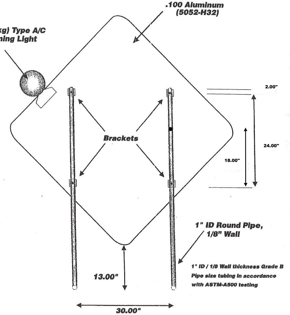
Back View
