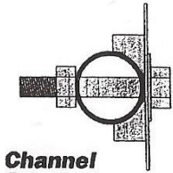
Channel Bracket Detail
